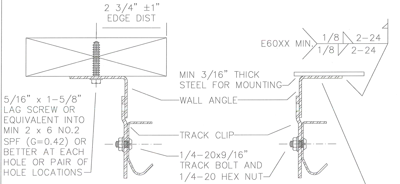
MOUNTING TO WOOD JAMB DETAIL
